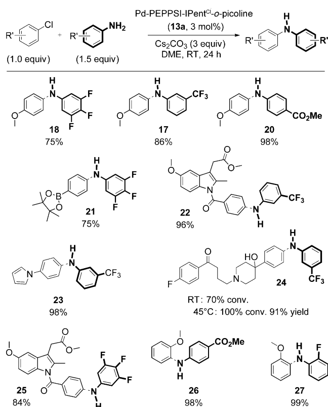
Scheme 3. Substrate scope of the room-temperature aryl aminations catalyzed by Pd-PEPPSI-IPent Cl - o -picoline ( 13a ). Reactions were conducted on a 0.5 mmol scale at a concentration of 1 M. Yields are reported for products purified by flash chromatography and were averaged over two runs.
